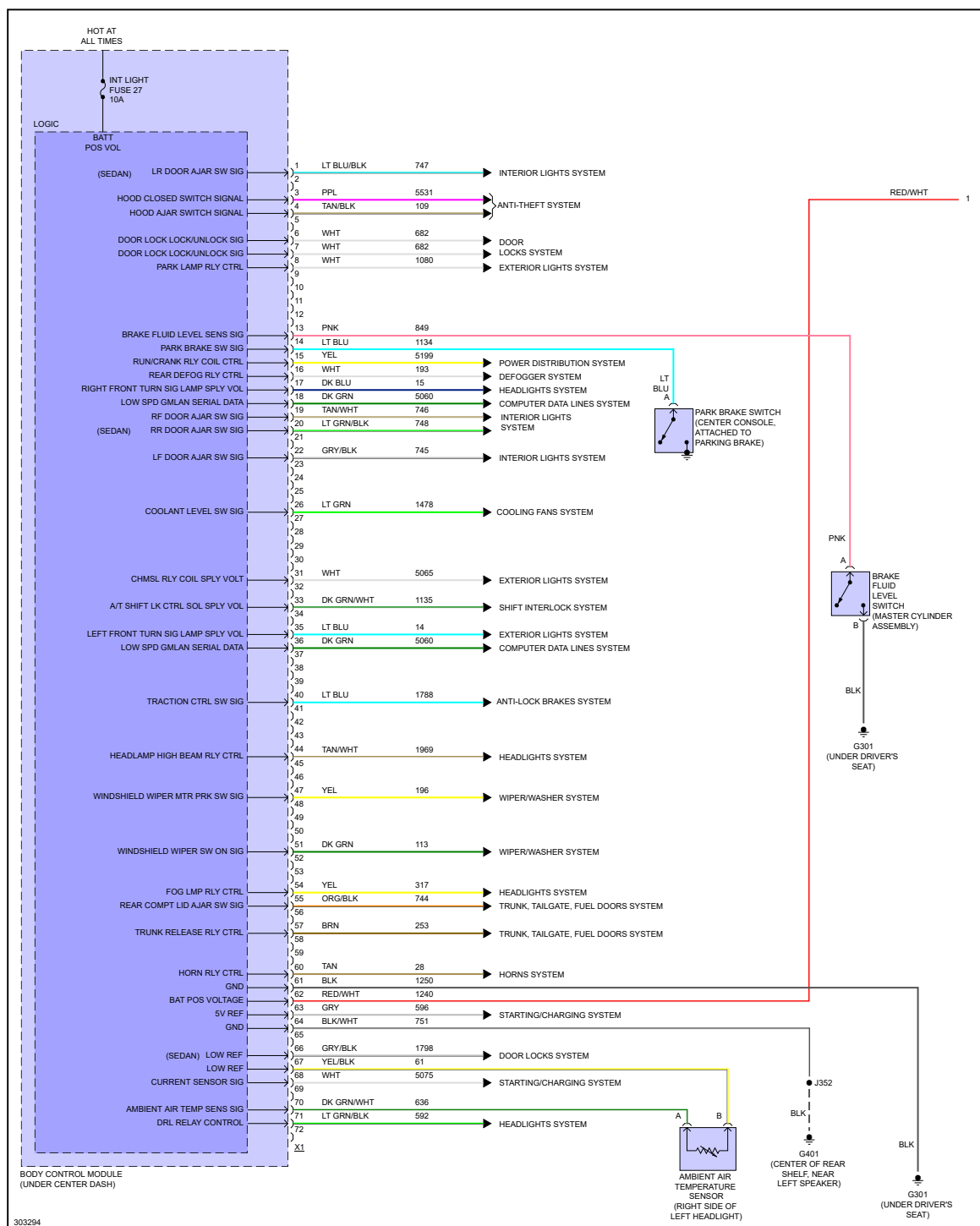
Fig 1: Body Control Modules Circuit (1 of 4)
