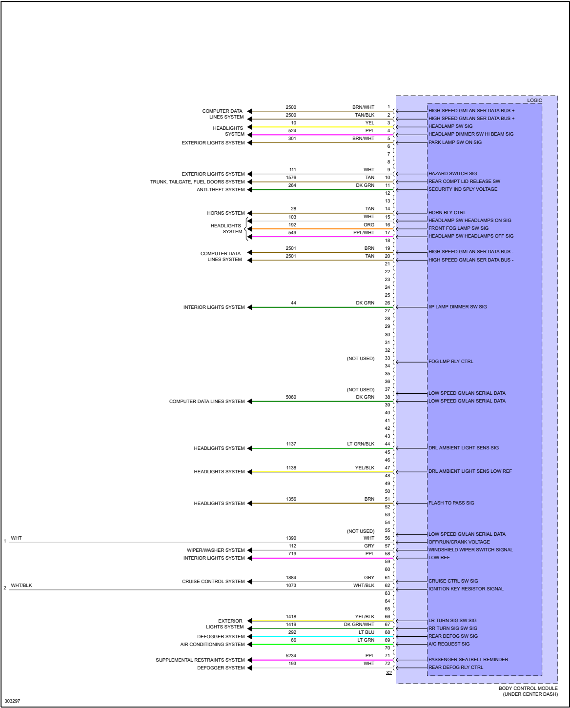
Fig 4: Body Control Modules Circuit (4 of 4)
