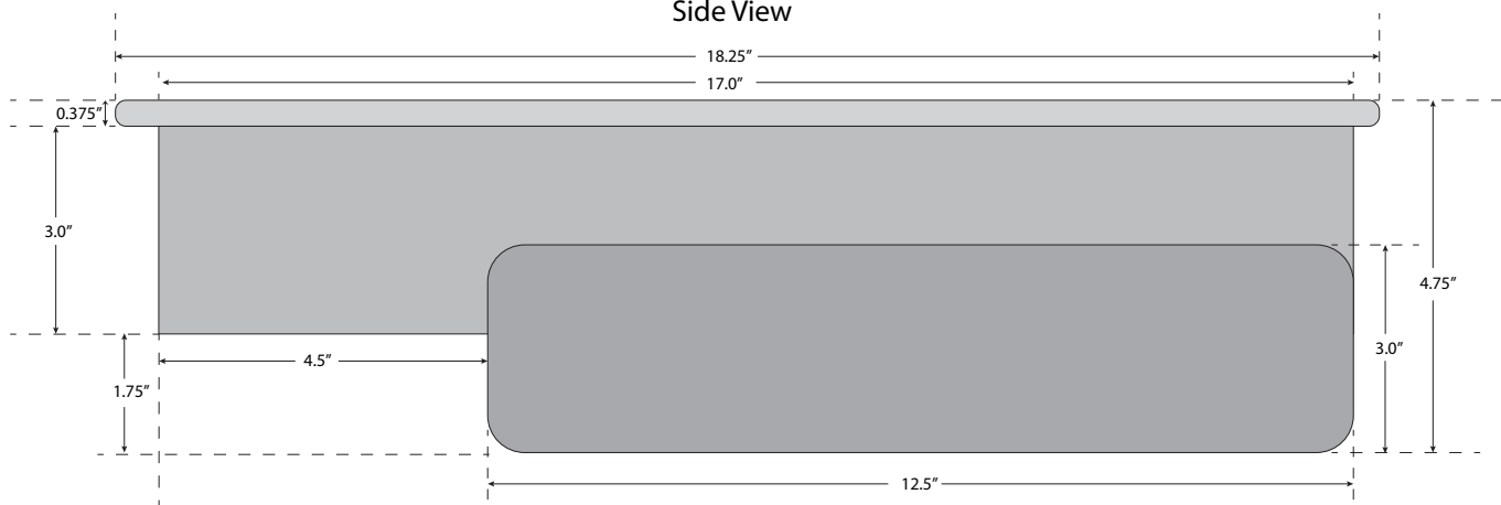
Side View
