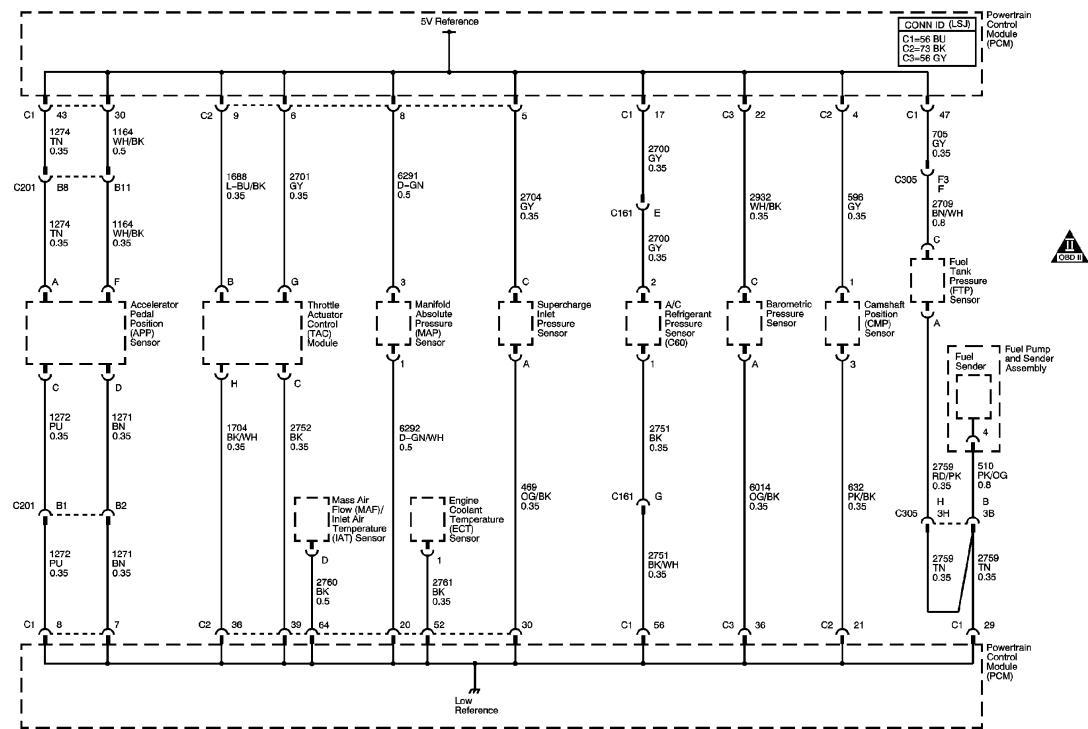
Engine Data Sensors – 5-Volt and Low Reference Bussing
