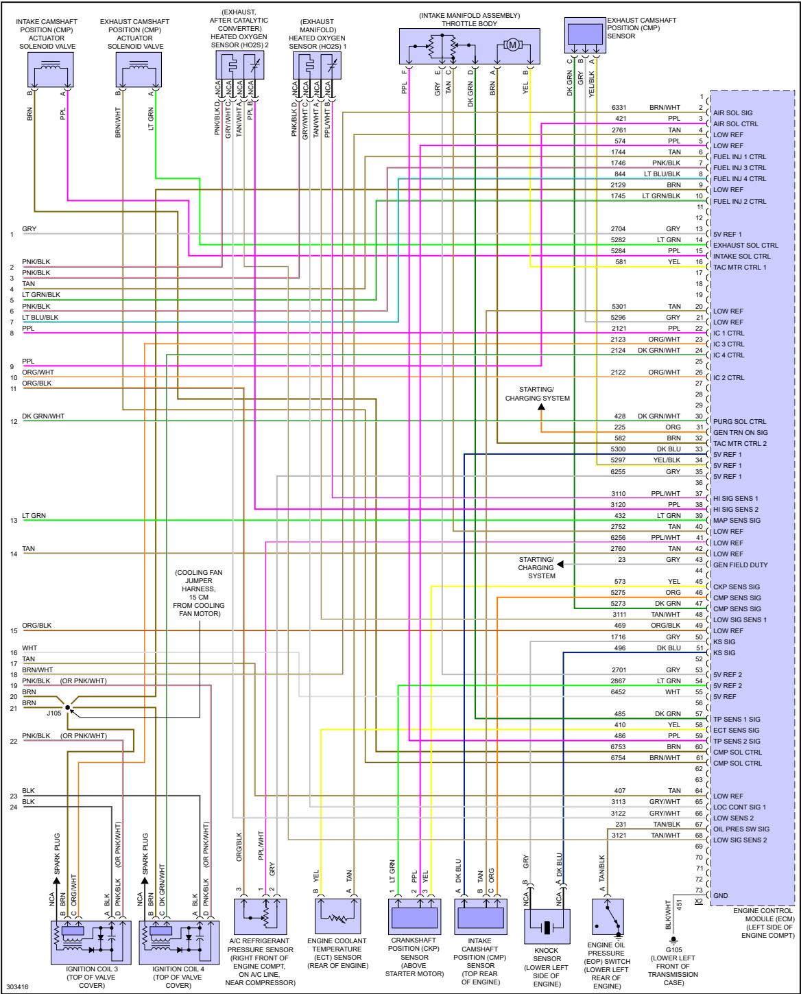
Fig 4: 2.2L VIN 5, Engine Performance Circuit (4 of 4)
