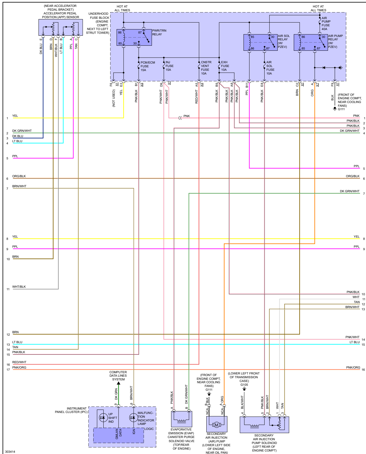
Fig 2: 2.2L VIN 5, Engine Performance Circuit (2 of 4)
