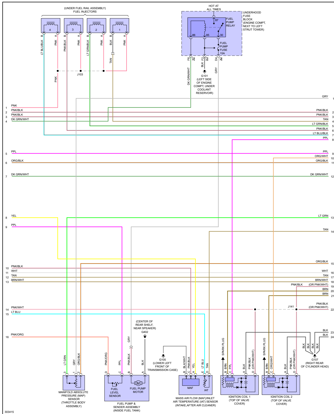
Fig 3: 2.2L VIN 5, Engine Performance Circuit (3 of 4)
