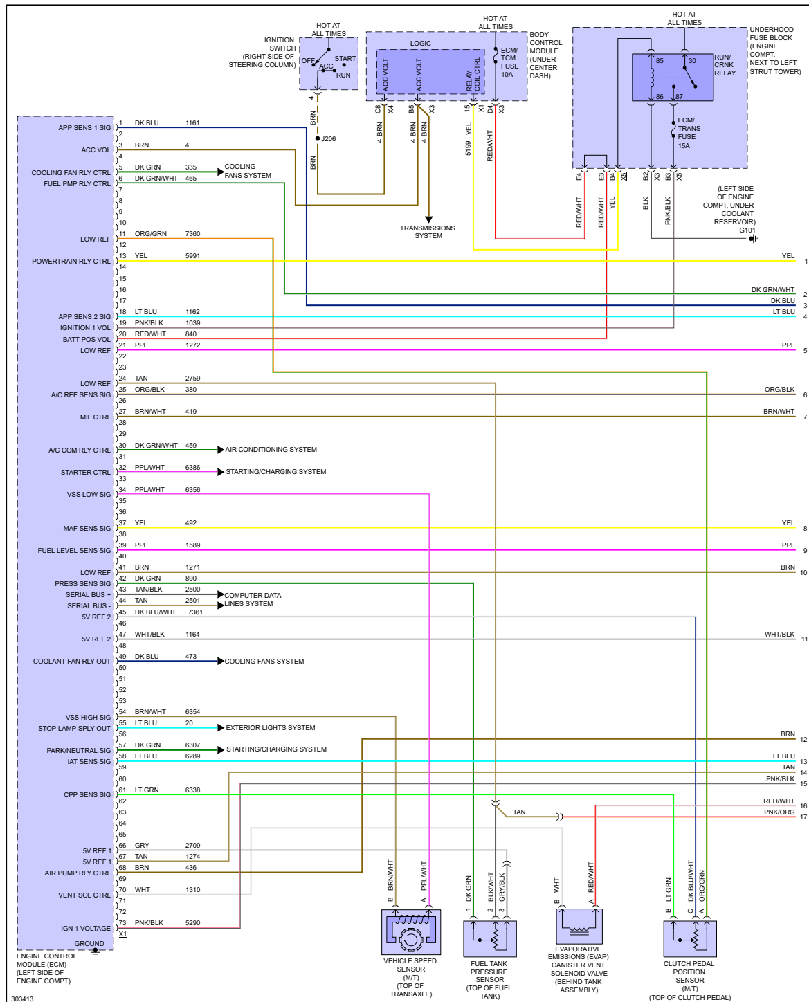
Fig 1: 2.2L VIN 5, Engine Performance Circuit (1 of 4)
