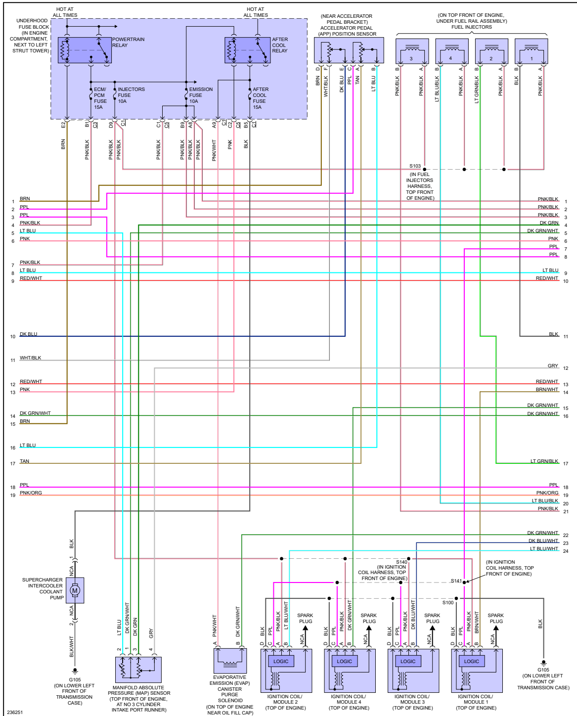
Fig 2: 2.0L VIN P, Engine Performance Circuit (2 of 4)
