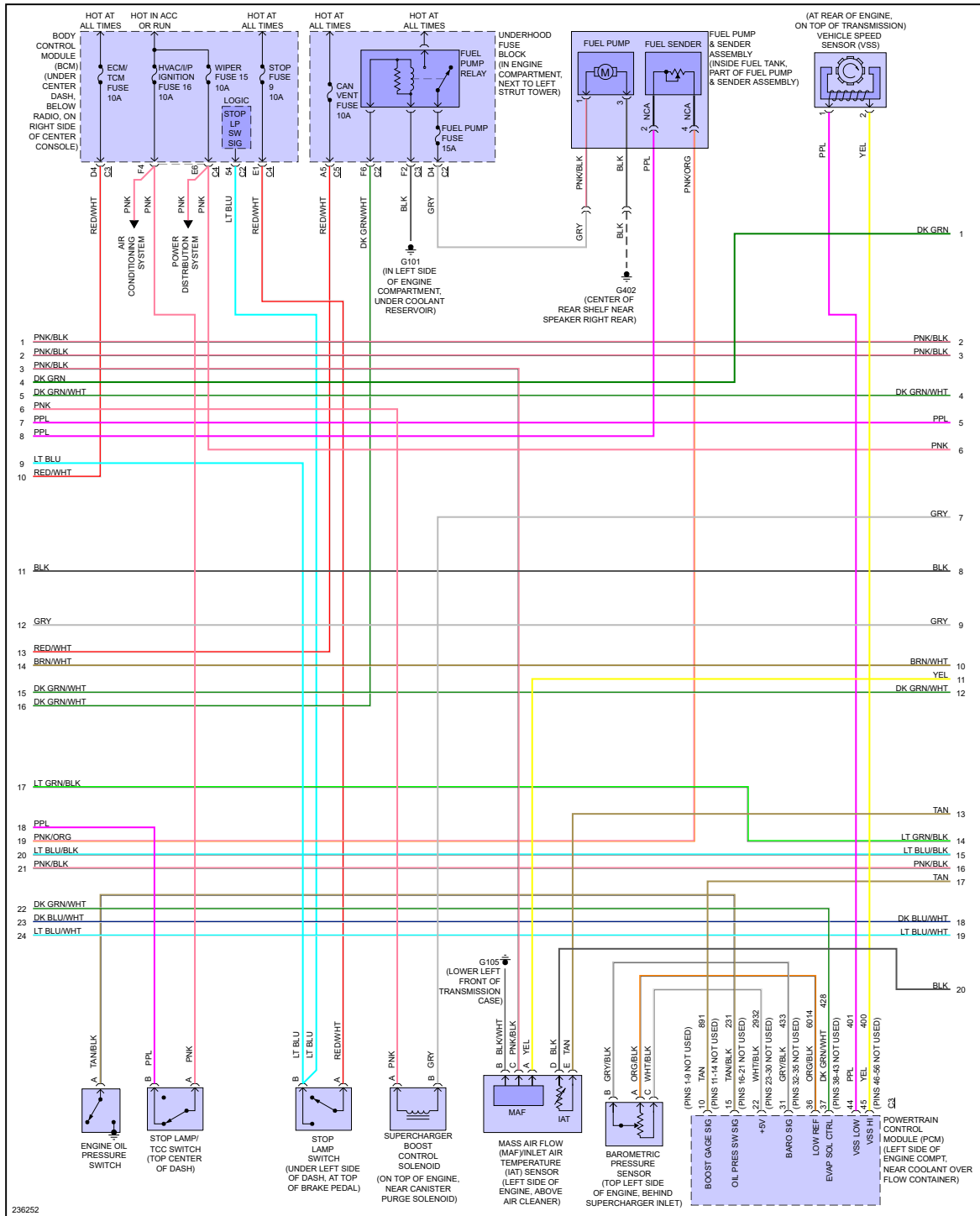
Fig 3: 2.0L VIN P, Engine Performance Circuit (3 of 4)
