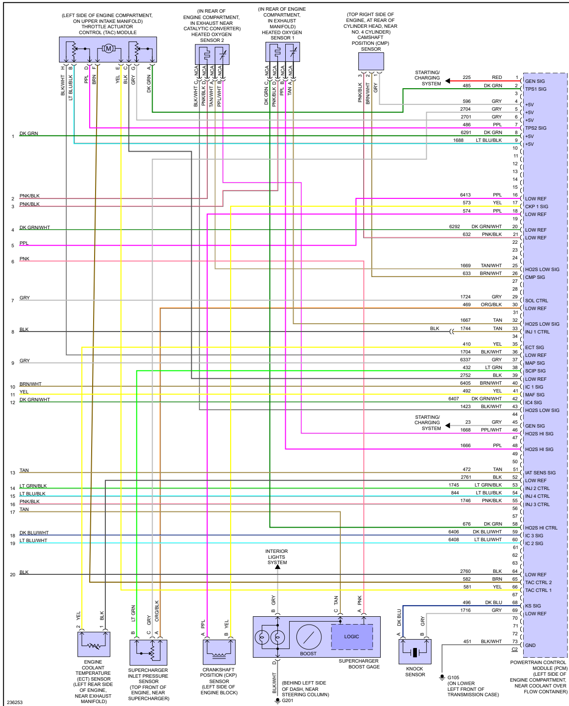
Fig 4: 2.0L VIN P, Engine Performance Circuit (4 of 4)
