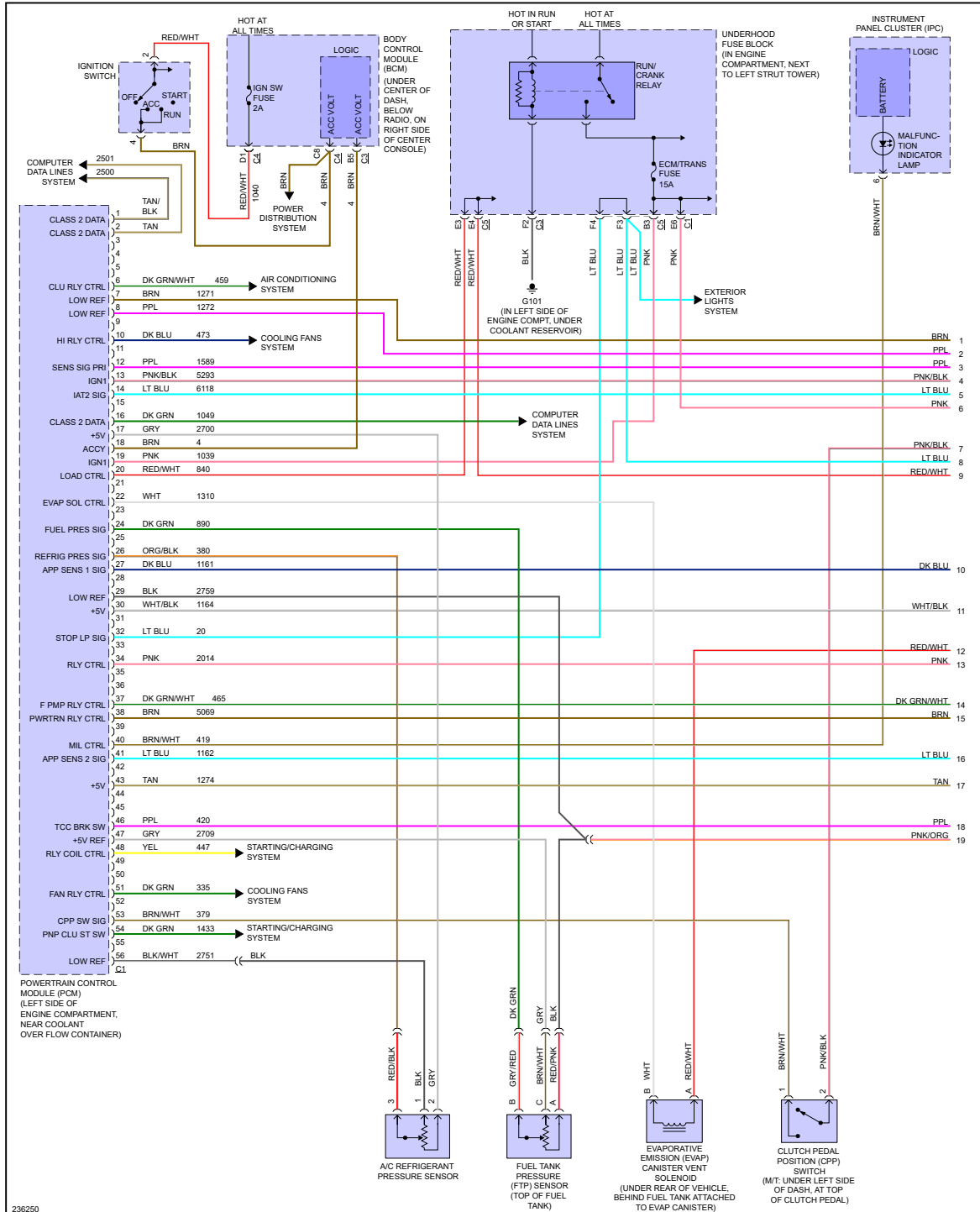
Fig 1: 2.0L VIN P, Engine Performance Circuit (1 of 4)
