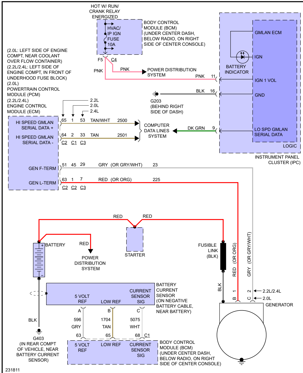
Fig 1: Charging Circuit
