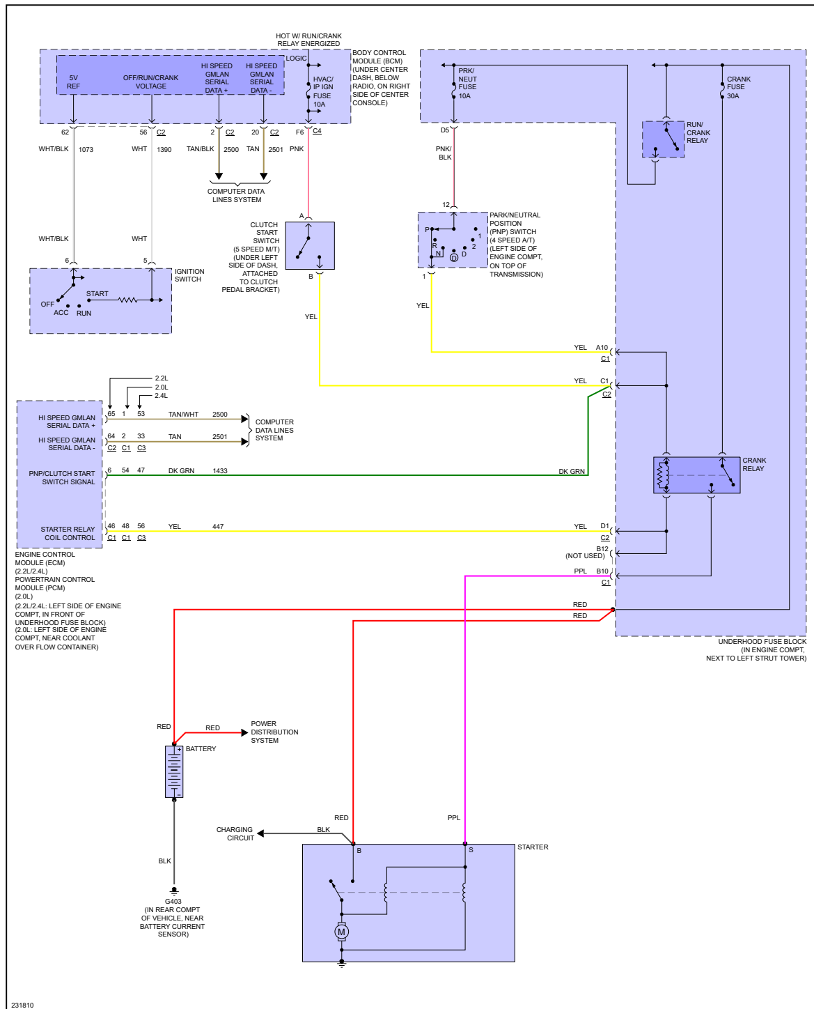
Fig 2: Starting Circuit
