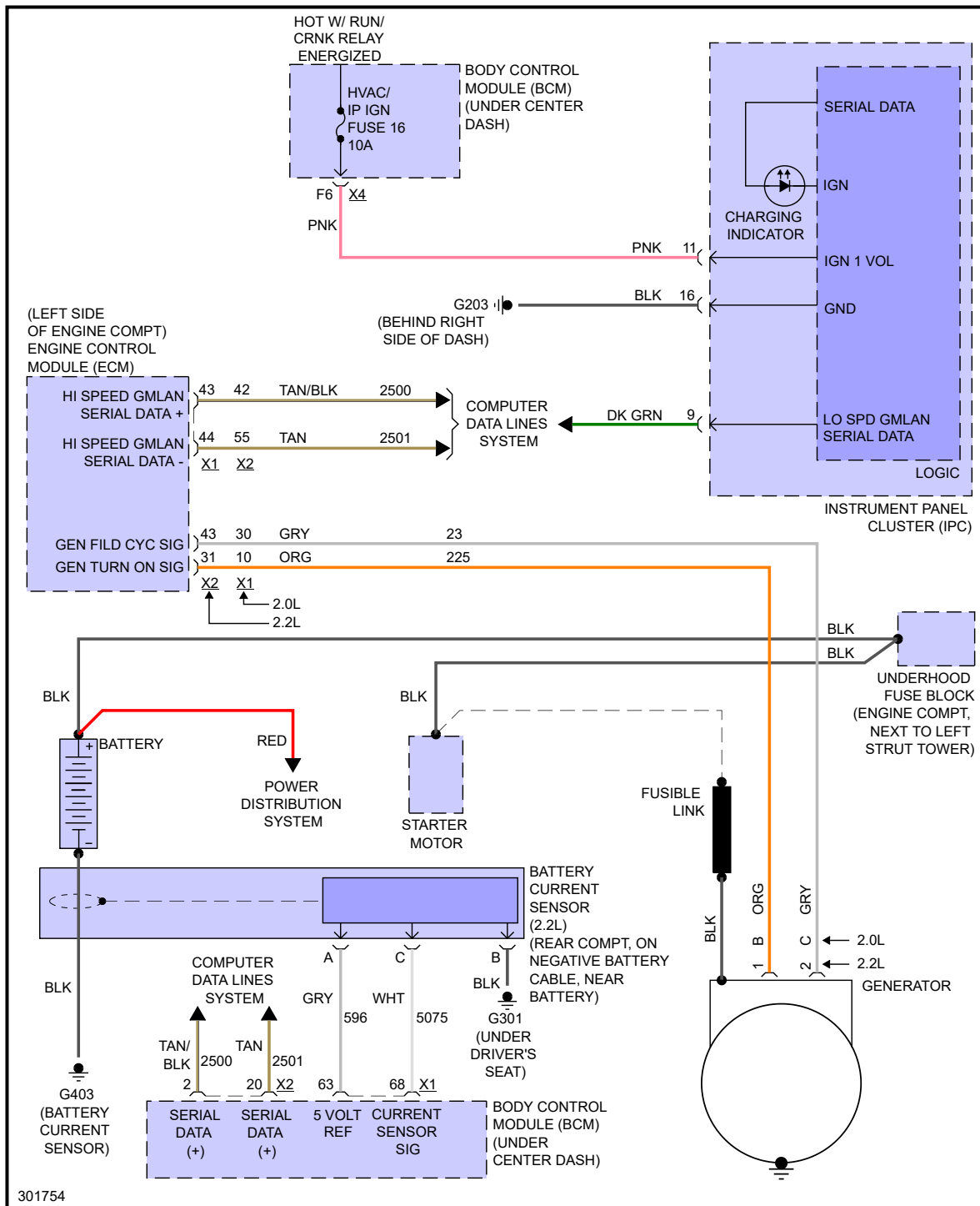
Fig 1: Charging Circuit
