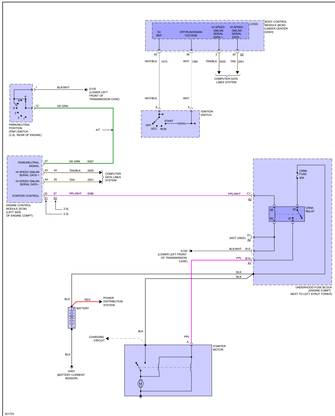
Fig 2: Starting Circuit
